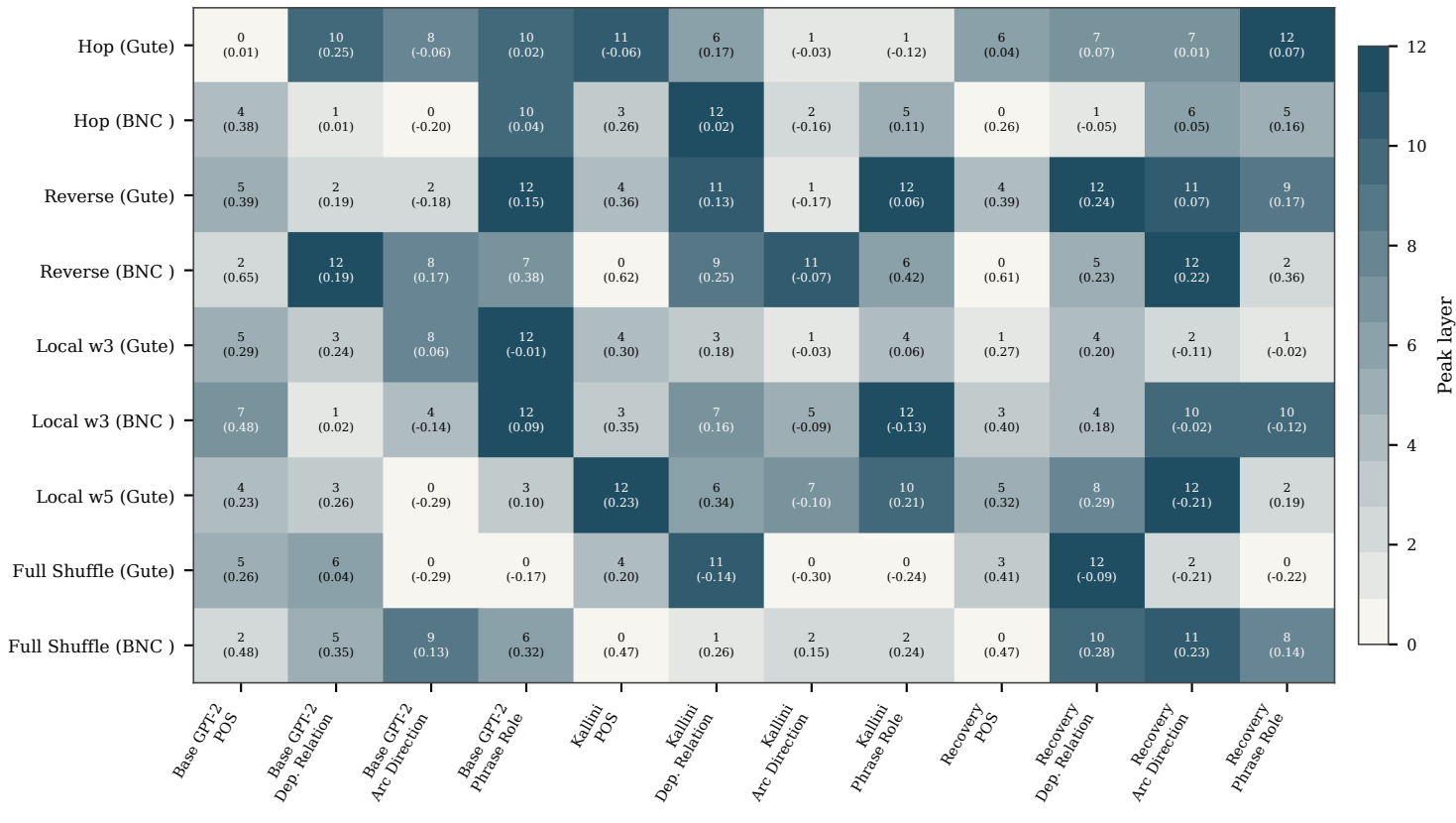
Peak V-information layer (Recovered)
